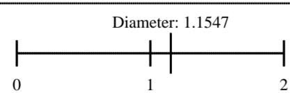
Title: Fullerene Net of HIV-1 Cone2 Source: Ganser, et al [1999] Faces: 178 Radius: 0.5774 Space: 0.0813 Date: Mar 2, 2014 By: Forrest McCluer, www.30computers.com
